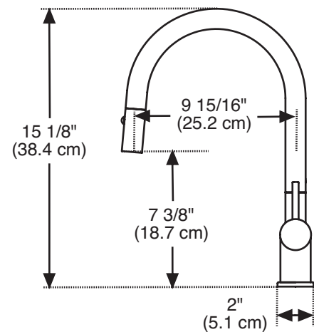
Dimensional Drawing
