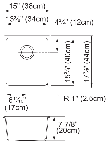
Dimensional Drawing
